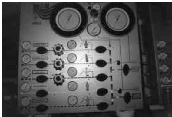
2 -diver mixed gas control panel.
